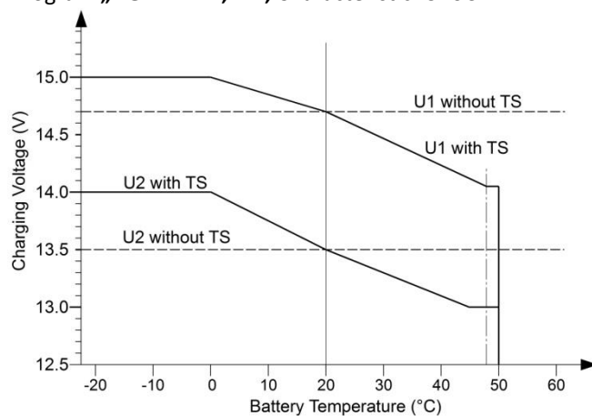
Program „AGM 2 14,4V“, Characteristic IU1oU2
