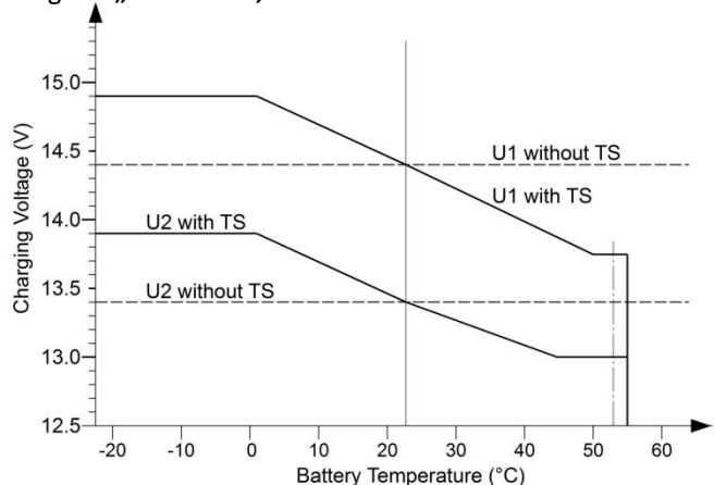
Program „Lead Acid“, Characteristic IU1oU2
