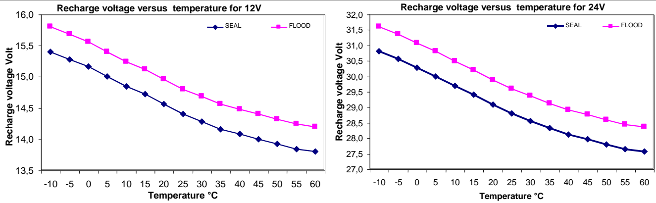
Pic. 6 Compensation curve of V_{ch} recharge voltage according to the battery temperature
