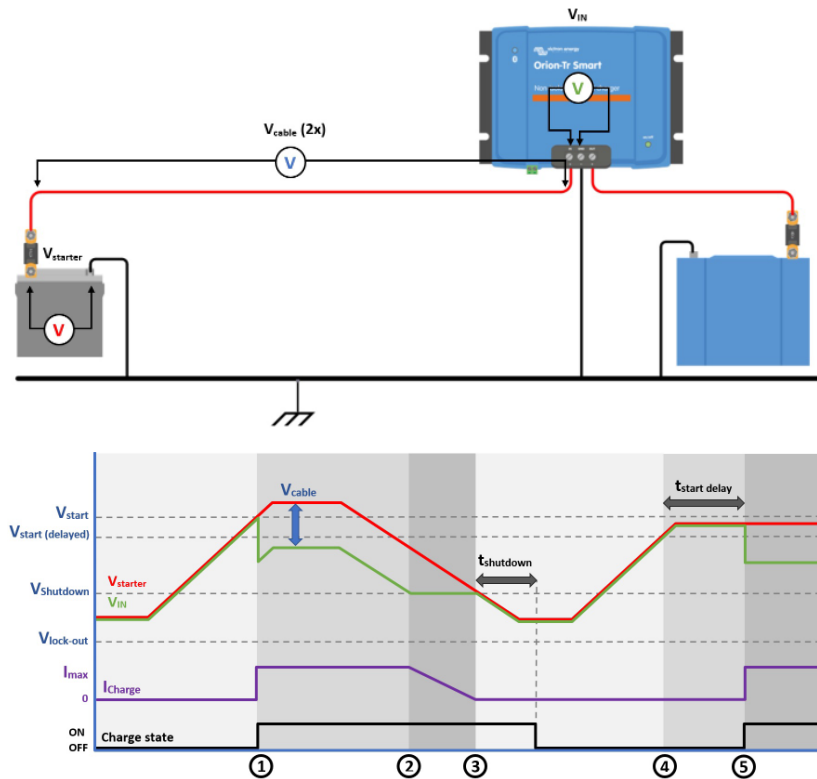
Figure 8: Engine shutdown detection sequence
