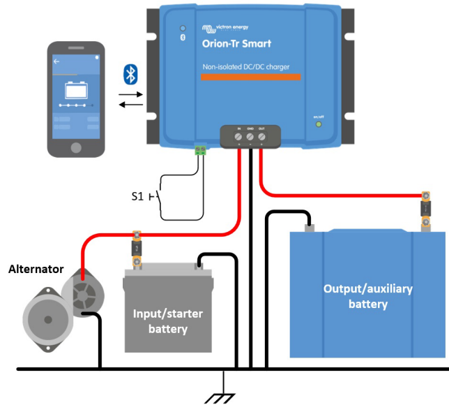
Figure 2: Typical connection setup as charger
