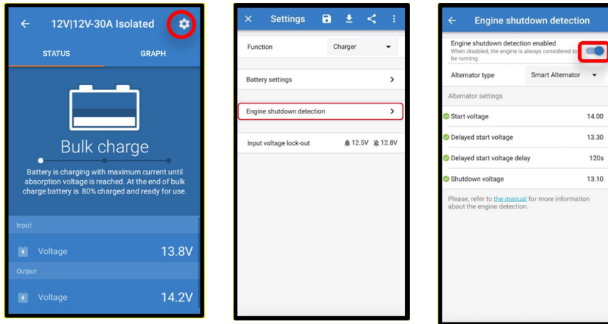
Figure 5: Disable engine shutdown detection
