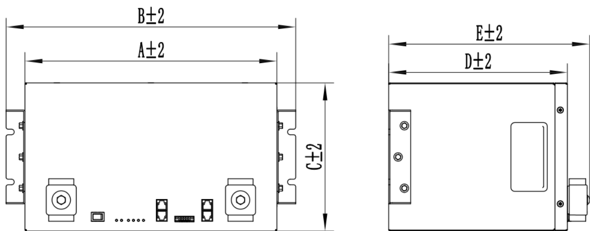
Figure 2-1 Picture of M12 lithium battery
