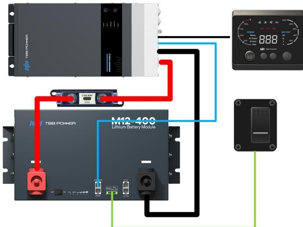
Figure 2-4b Typical wiring diagram 2 (with TBB inverter)
