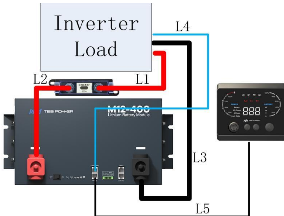
Figure 3-3a Typical wiring diagram 1 (non-TBB inverter)
