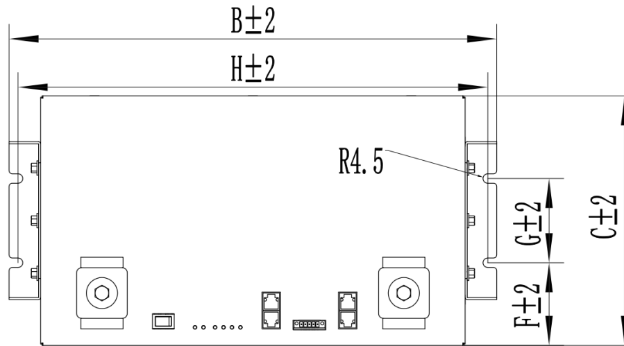
Figure 3-1 Installation positioning requirement
