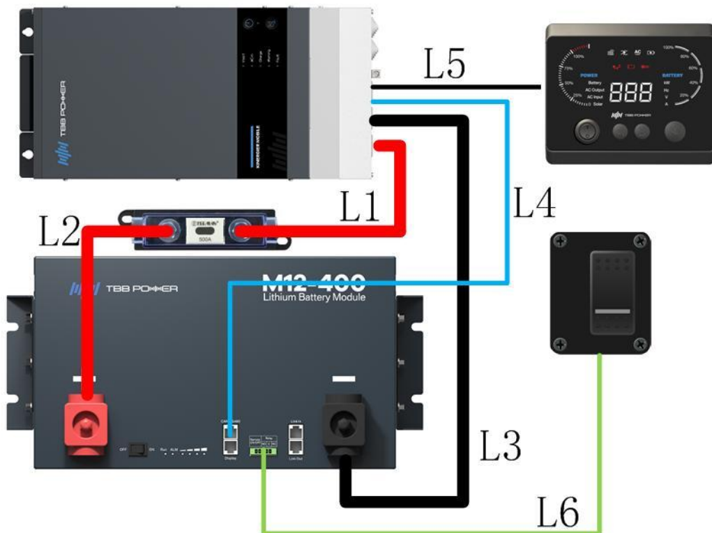
Figure 3-3b Typical wiring diagram 2 (TBB inverter)
