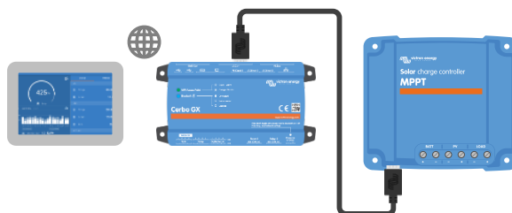
VictronConnect App connection via LAN or the internet (VRM portal) using a GX device (for example a Cerbo GX)
