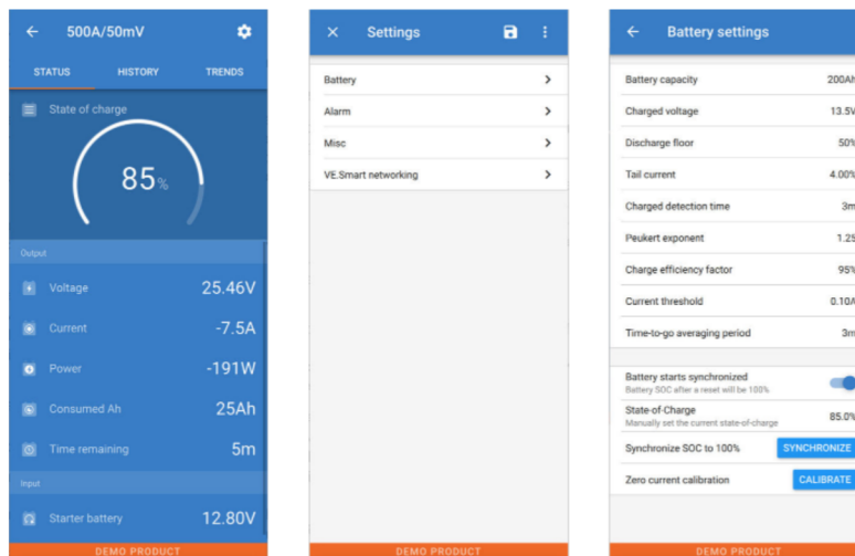
VictronConnect settings
